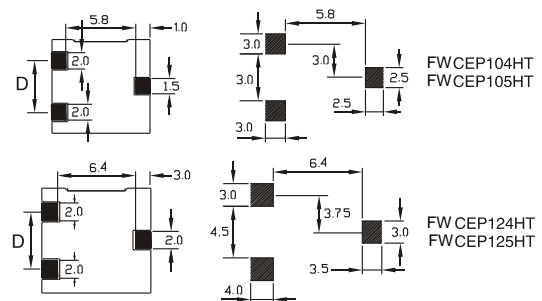
LAND PATTERN
